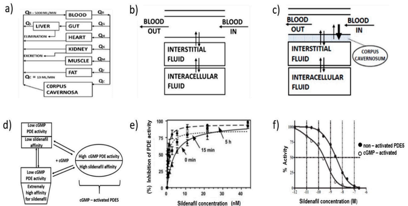
Figure 3. Pharmacodynamic profile of sildenafil: (a) distribution flows in a physiological map of human tissues; (b) schematic of artery and interstitial/intracellular medium, intracellular tissue; (c) schematic of artery and interstitial/intracellular medium, intracellular tissue pinpointing the corpus cavernosum compartment; (d) conversion of the catalytic center of the PDE5 enzyme into a higher affinity structure; (e) enhancement of inhibition of PDE activity by increase of sildenafil concentration (adopted from [40] with permissions) (f) differential affinities of sildenafil inhibition activated by cGMP (adopted from [42] with permissions).
