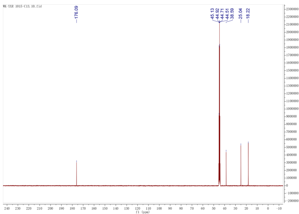
Fig 2 13 C NMR spectrum of Butyrimidamide hydrochloride
