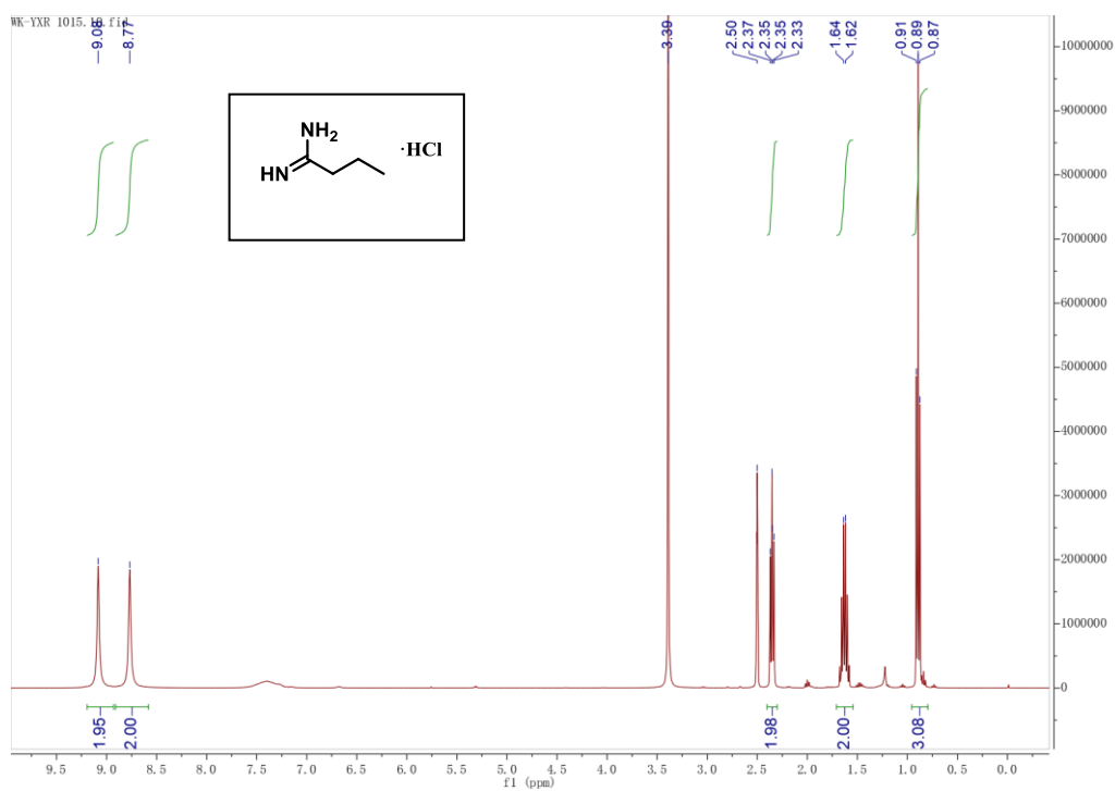
Fig 1 1 H NMR spectrum of Butyrimidamide hydrochloride
